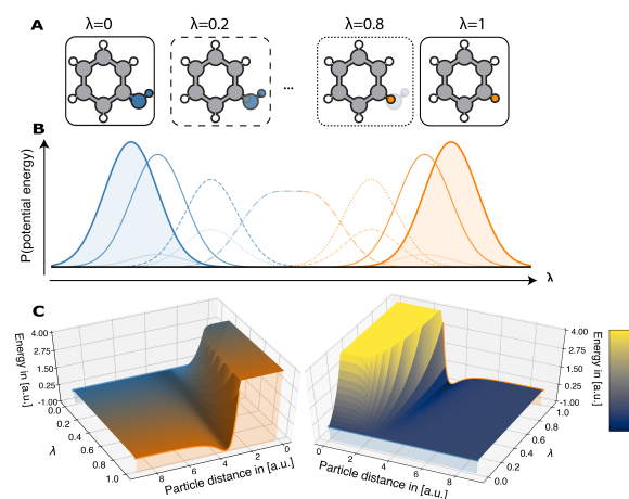
Figure 7. Alchemical intermediates are created by making the potential energy depend on an additional variable \lambda that interpolates between the chemical endpoints. In (A), at \lambda = 0 the molecule is a fully interacting phenol and at \lambda = 1 , a fully interacting benzene. (B) shows an illustration of the probability distribution of the potential energies as the switching function takes values of \lambda = 0 to \lambda = 1 . Intermediate states are required for a sufficient overlap in potential energies to estimate a free energy difference between \lambda = 0 and \lambda = 1 . Soft-core potentials provide one of the most efficient families of intermediate pathways, with a \lambda dependence. In (C) the potential energy surface is coloured according to \lambda with blue being \lambda = 0 and \lambda = 1 orange. In (D) the potential is coloured according to the potential energy. Note how as \lambda approaches 0, the energy smoothly approaches zero at all r , a necessary requirement for efficient and stable calculations.
