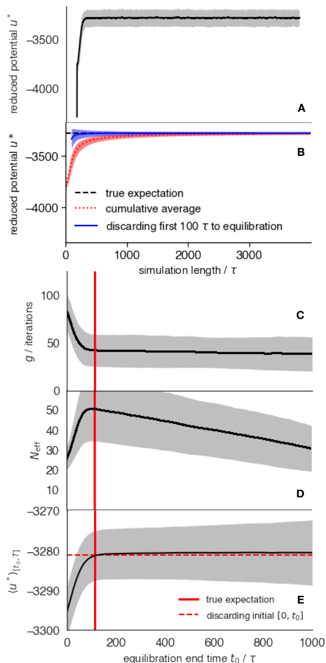
Figure 11. Automatic partitioning into equilibration and production regions. (A) The average (black line) standard deviation (shaded region) of the reduced potential U^* over many independent replicate simulations started from the same initial conditions show a significant initial transient change before relaxing to the true average potential energy (B). A cumulative average (red) of the entire simulation data demonstrates simulation bias not seen when initial simulation data is omitted (blue). Using an automated approach to detect equilibration of the boundary t_0 using statistical inefficiency g (C) for an effective simulation interval (D). (E) The optimal equilibration boundary t_0 is selected to maximize the number of uncorrelated samples. Figure adapted from [210].
