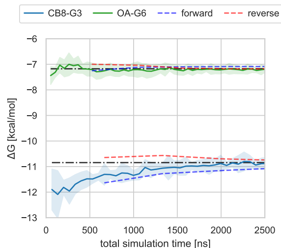
Figure 12. Average binding free energy of 5 replicate Hamiltonian replica exchange calculations as a function of total simulation time (i.e. the sum of the simulation time of all replicas) for the two host-guest systems CB8-G3 and OA-G6. Shaded areas represent 95% confidence intervals around the mean computed from the 5 replicates data. The horizontal dash-dot lines show the final binding free energy prediction of the two calculations after a total of 5230 ns for OA-G6 and 6650 ns for CB8-G3. Dashed lines are the free energy trajectories computed in the forward (blue) and reverse (red) time direction for a single replicate calculation. Longer correlation times in CB8-G3 cause the calculation to converge more slowly. The original data used to generate the plot can be found at https://github.com/samplchallenges/SAMPL6/blob/master/host_guest/Analysis/SAMPLing/Data/reference_free_energies.csv .
