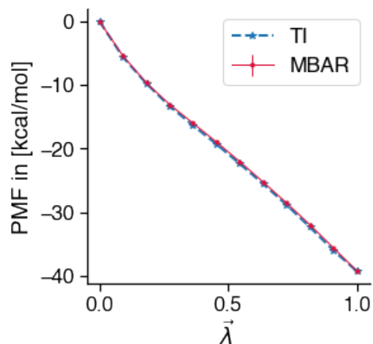
Figure 10. Potential of mean force with respect to \bar{\lambda} for TI and MBAR The estimated PMF for a bound calculation of a Tyk2 ligand pair of Wang et al. [15] with respect to \bar{\lambda} estimated from TI and MBAR and showing agreement within errorbars.
