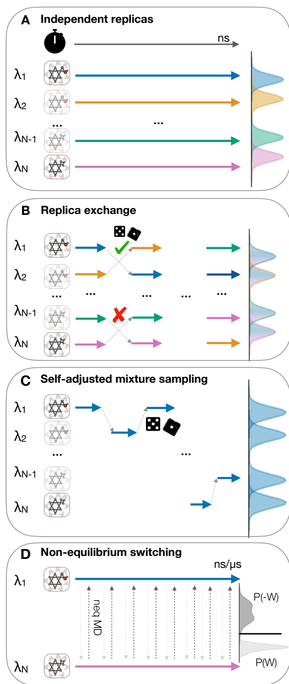
Figure 8. Four most common sampling strategies. (A): Multiple replicas in parallel at different lambda states. Each arrow symbolises an independent \bar{\lambda} simulation. (B): Hamiltonian replica exchange scheme. Each arrow represents a short simulation interval before an exchange through Metropolis Hastings acceptance (dice) is attempted. A tick means an accepted exchange, a cross a rejected exchange. (C): Single replica scheme sampling from all \bar{\lambda} states. After a short simulation time symbolised by the arrow, the lambda-state is attempted to change until all N lambda states will be sampled. (D): Non-equilibrium sampling scheme, where two equilibrium simulations at the end states are run as indicated by the blue and pink arrow. Non-equilibrium simulations are attempted at intervals to switch between the two end states.
