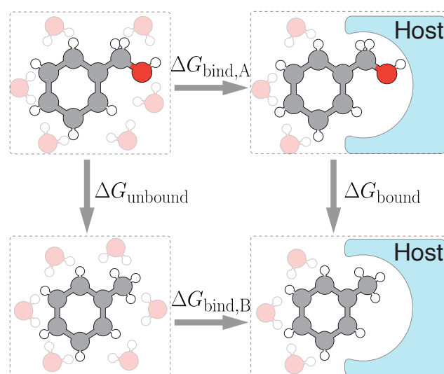
Figure 2. Thermodynamic cycle for computing the relative free energy of binding ( \Delta\Delta G ) between two related small molecules to a supramolecular host or a rigid receptor. The relative binding free energy difference between two small molecules, \Delta\Delta G_{\text{bind},A \rightarrow B} \equiv \Delta G_{\text{bind},B} - \Delta G_{\text{bind},A} —here benzyl alcohol (top) to toluene (bottom)—can be computed as a difference between two alchemical transformations, \Delta G_{\text{bound}} - \Delta G_{\text{solvated}} , where \Delta G_{\text{bound}} represents the free energy change of transforming A \rightarrow B in complex, i.e. bound to a host molecule, and \Delta G_{\text{unbound}} the free energy change of transforming A \rightarrow B in solvent, typically water.
