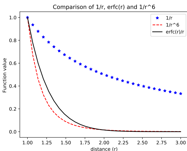
Figure 7. Comparison of decay of the original r^{-1} term for Coulomb interactions (blue,*) , the resulting direct-space term after Gaussian screening (black,-) and the r^{-6} in van der Waals term (red, -). Note: The value on the vertical axis has been scaled to allow easy visualization of the relative decay of each term.
